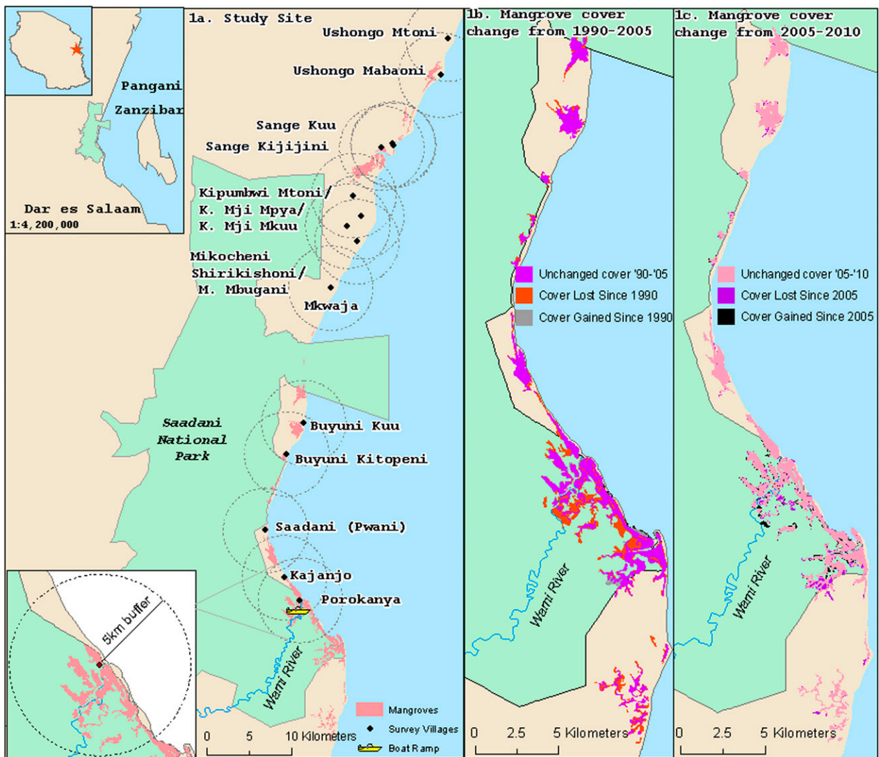
Fig. 1. (A) Study site of SANAPA, Tanzania, and villages used in econometric analyses. Inset : 5-km radius around each village used to assess mangrove cover change per village within and outside SANAPA. (B and C) Change in mangrove forest cover from 1990 to 2005 (B) and from 2005 to 2010 (C).
